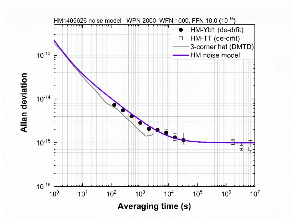
Figure 1. Frequency instability of the hydrogen maser (HM1405626)
