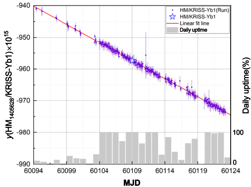
Figure 1. The violet points are averaged data of y(\text{HM}_{1405628}/\text{KRISS-Yb1}) \times 10^{15} over around 4,000 s with each uncertainty. The blue star indicates the determined value of y(\text{HM}_{1405628}/\text{KRISS-Yb1}) . The red line is the linear fit (drift rate : -1.145 \times 10^{-15}/\text{d} ). The grey bars represent the daily uptime of KRISS-Yb1.
