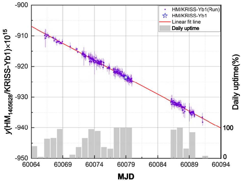
Figure 1. The violet points are averaged data of y(\text{HM}_{1405628}/\text{KRISS-Yb1}) over 3,000~12,000 s with each uncertainty. The blue star indicates the determined value of y(\text{HM}_{1405628}/\text{KRISS-Yb1}) . The red line is the linear fit (drift rate : -1.1 \times 10^{-15}/\text{d} ). The grey bars represent the daily uptime of KRISS-Yb1.
