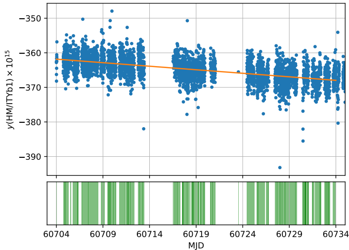
Figure 1: Fractional frequency deviation y(\text{HM1401103}/\text{ITYb1}) measured in the period MJD 60704 - 60734. Green shaded regions in the bottom plot represent the uptime of IT-Yb1.
