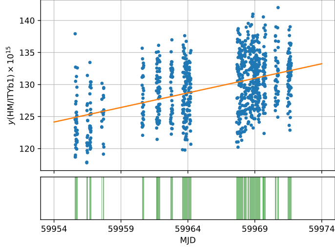
Figure 1: Fractional frequency deviation y(\text{HM1401104}/\text{ITYb1}) measured in the period MJD 59954 - 59974. Green shaded regions in the bottom plot represent the uptime of IT-Yb1.
