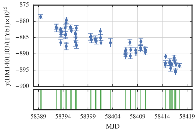
Figure 1: Fractional frequency deviation y(\text{HM1401103}/\text{ITYb1}) measured in the period MJD 58389 - 58419. Green shaded regions in the bottom plot represent the uptime of IT-Yb1.
