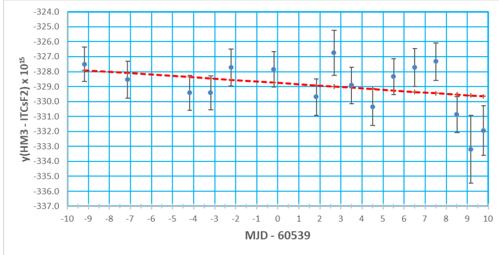
Figure 3. y(HM3-ITCsF2) data and the linear fit curve centered in MJD 60539
