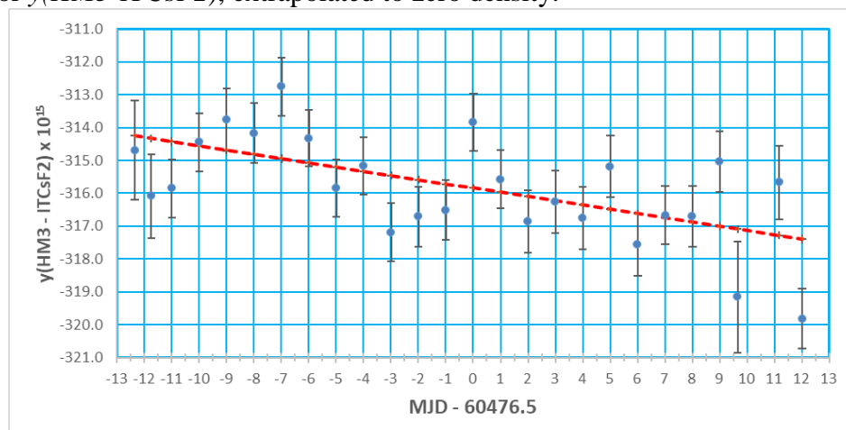
Figure 3. y(\text{HM3-ITCsF2}) data and the linear fit curve centered in MJD 60476.5
