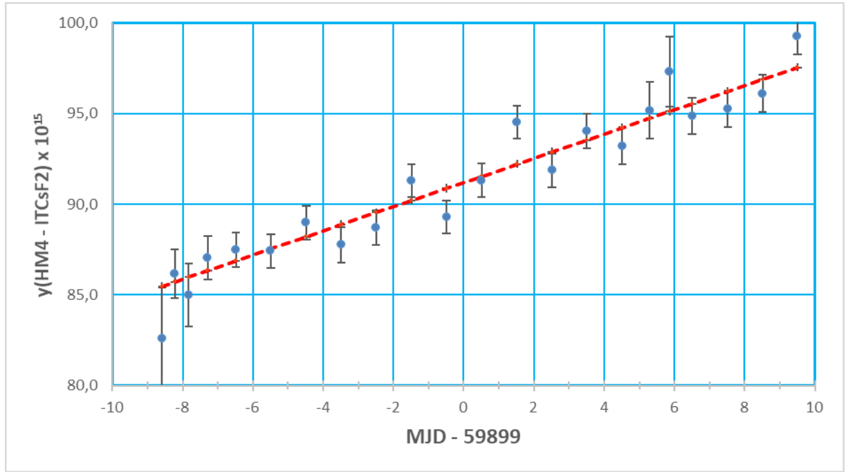
Figure 3. y(HM4-ITCsF2) data and the linear fit curve centered in MJD 59899
