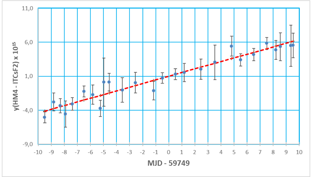
Figure 3. y(HM4 - ITCsF2) data and the linear fit curve centered in MJD 59749
