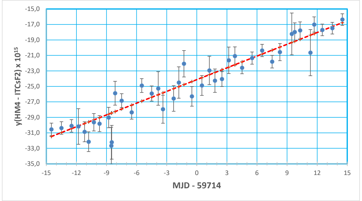
Figure 3. y(HM4 - ITCsF2) data and the linear fit curve centered in MJD 59714
