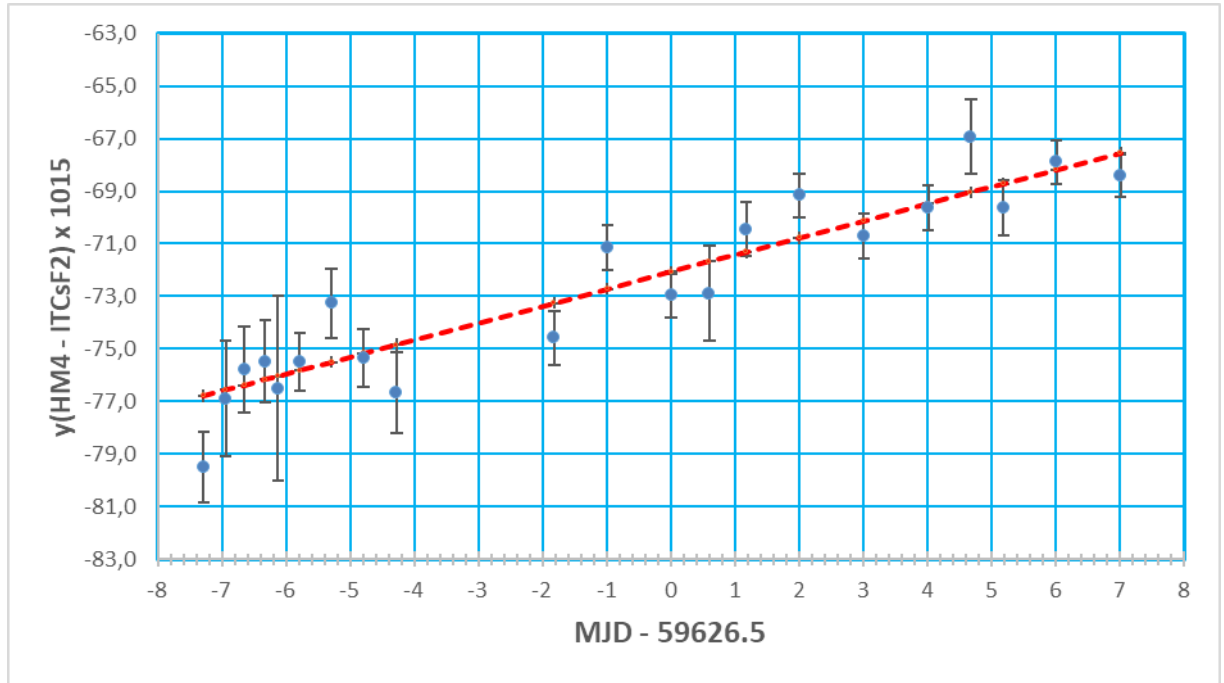
Figure 3. y(HM4-ITCsF2) data and the linear fit curve centered in MJD 59626.5
