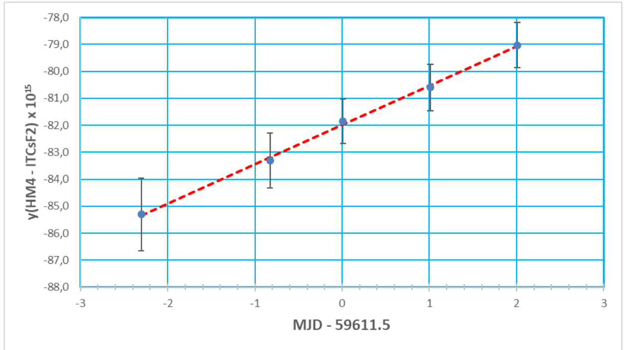
Figure 3. y(HM4-ITCsF2) data and the linear fit curve centered in MJD 59611.5
