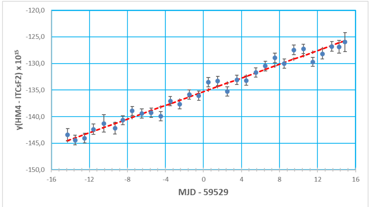
Figure 3. y(HM4-ITCsF2) data and the linear fit curve centered in MJD 59529
