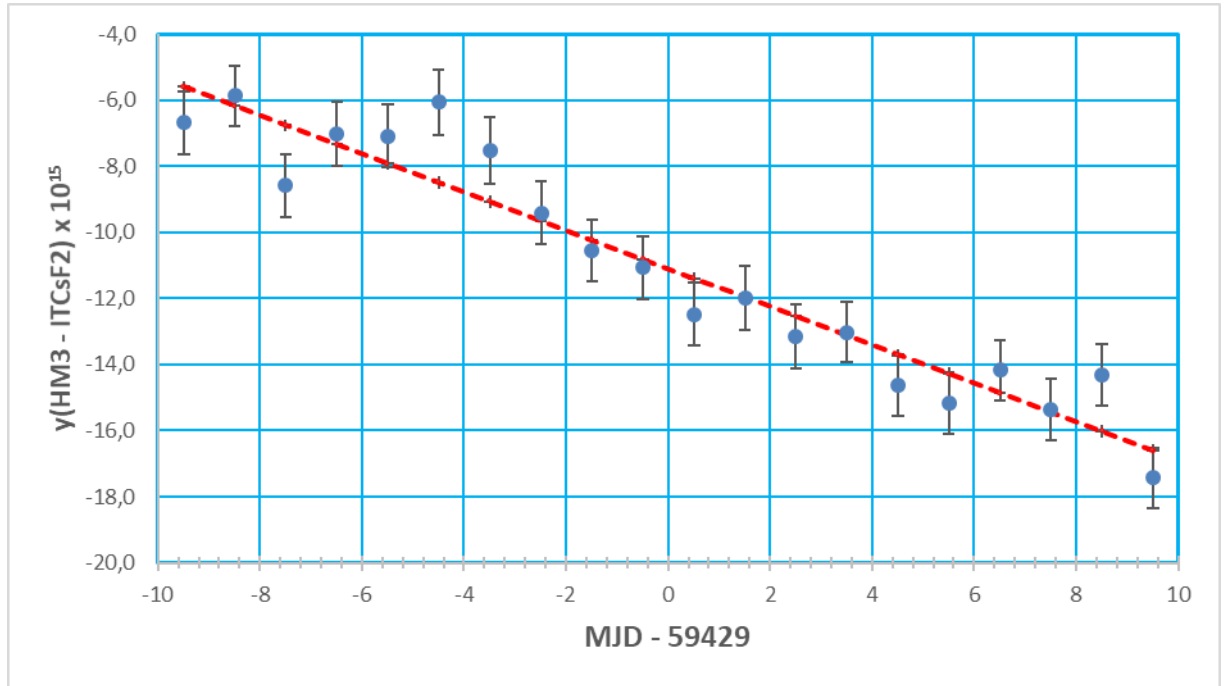
Figure 3. y(HM3-ITCsF2) data and the linear fit curve centered in MJD 59429
