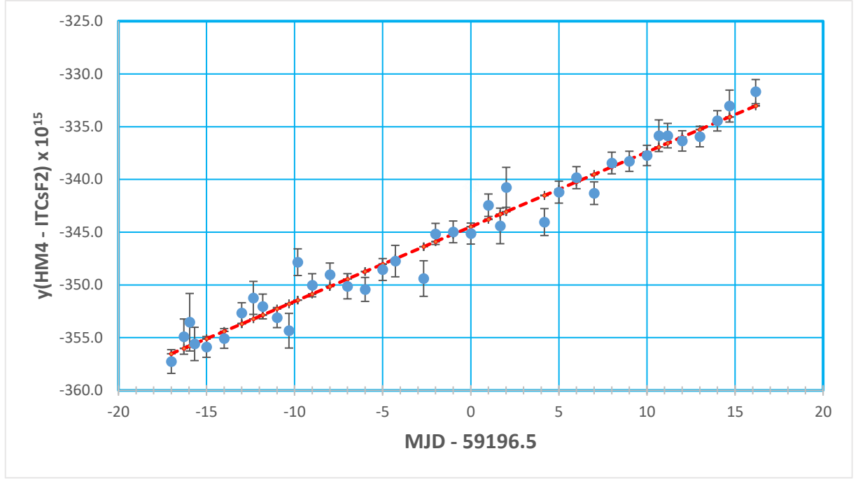
Figure 3. y(HM4-ITCsF2) data and the linear fit curve centered in MJD 59196.5
