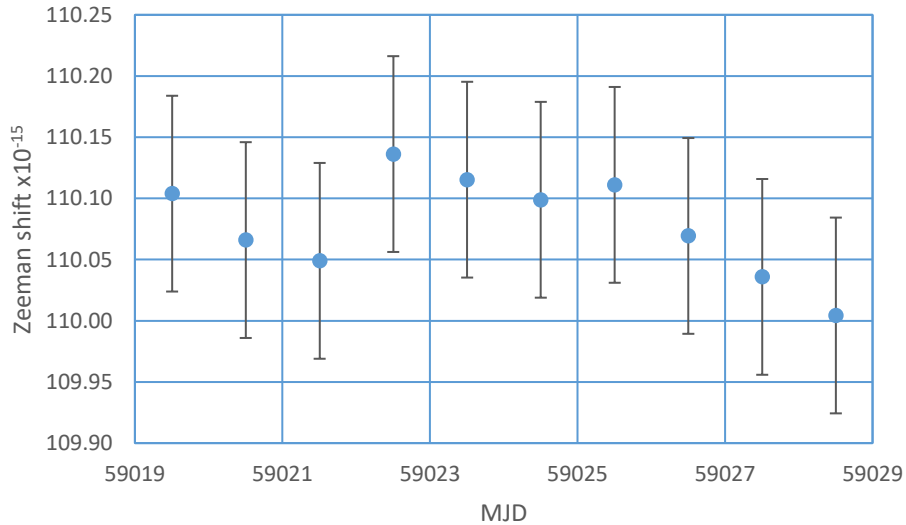
Figure 1. Zeeman shift fluctuations during the TAI evaluation period.
