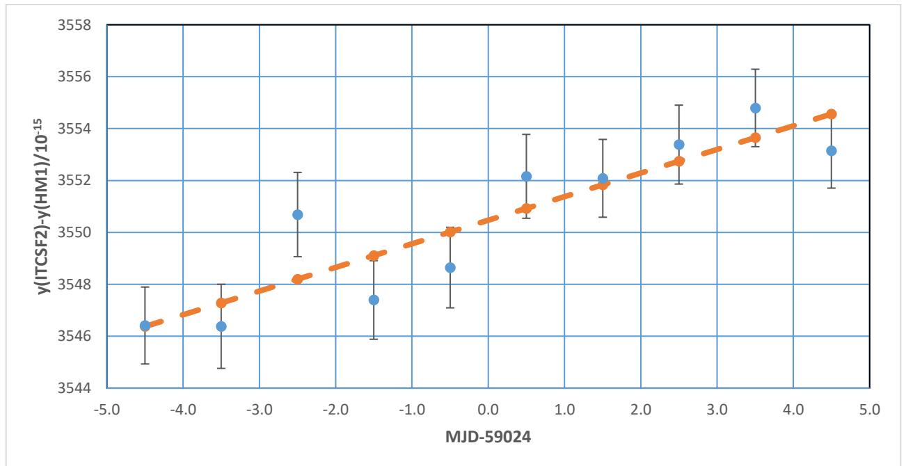
Figure 2. y(ITCsF2) - y(HM1) data and the linear fit curve centered in 59024.
