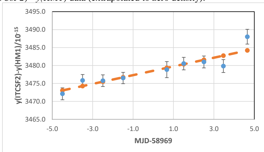
Figure 3. y(ITCsF2) - y(HM1) - data and the linear fit curve.
