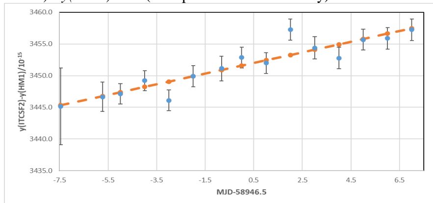
Figure 3. y(ITCsF2) - y(HM1) - data and the linear fit curve.
