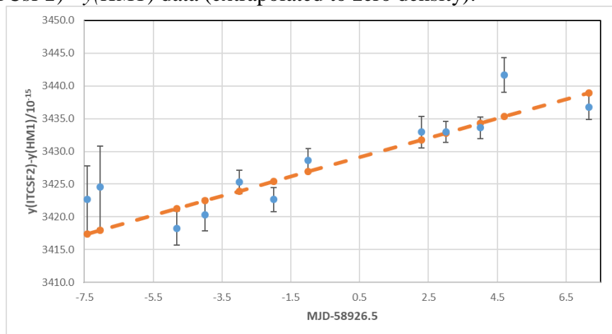
Figure 3. y(ITCsF2) - y(HM1) - data and the linear fit curve.
