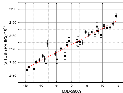
Figure 3. y(ITCsF2) - y(HM2) - data and the linear fit curve.
