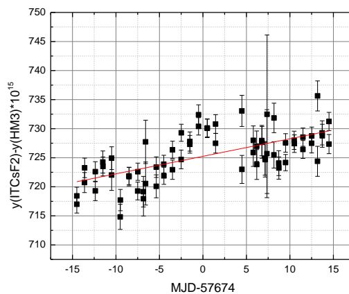
Figure 3. y(ITCsF2) - y(HM3) - data and the linear fit curve.
