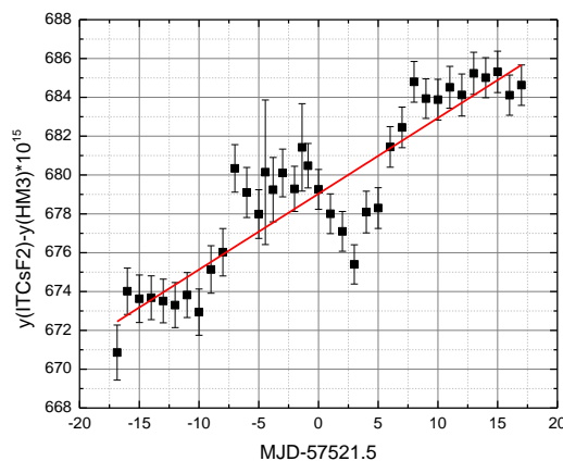
Figure 3. y(ITCsF2) - y(HM3) - data and the linear fit curve.
