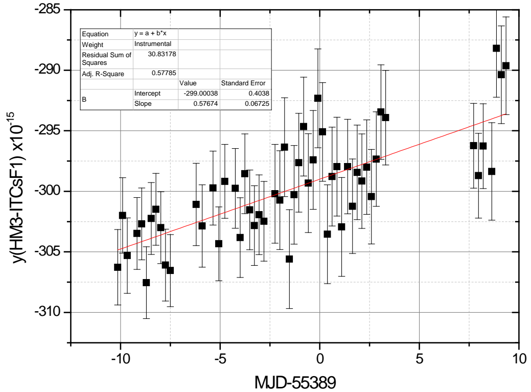
Figure 3. y(HM3) - y(IT-CsF1) data and the Bayesian linear fit curve (straight line).
