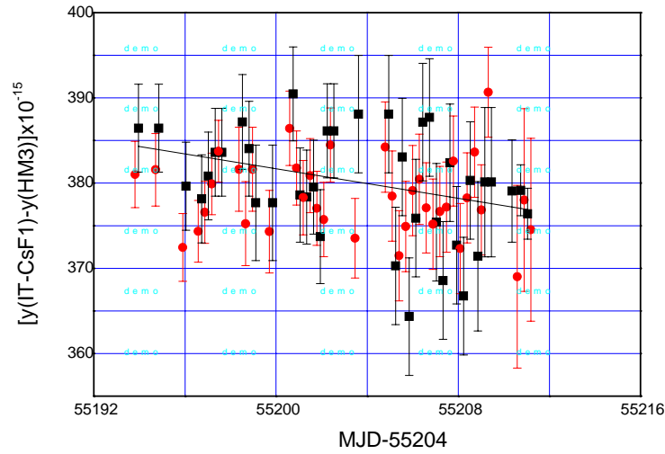
Figure 4. y(HM3) - y(IT-CsF1) data and the Bayesian linear fit curve (straight line).
