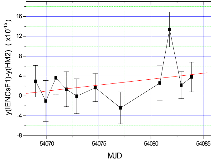
Figure 3. y(IEN-CsF1)-y(HM2) data (squares) and the linear fit curve (straight line).
