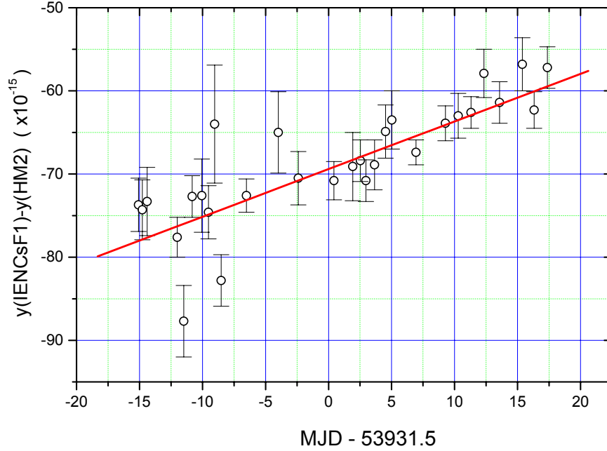
Figure 3. y(IEN-CsF1)-y(HM2) data (circles) and the linear fit curve (straight line).
