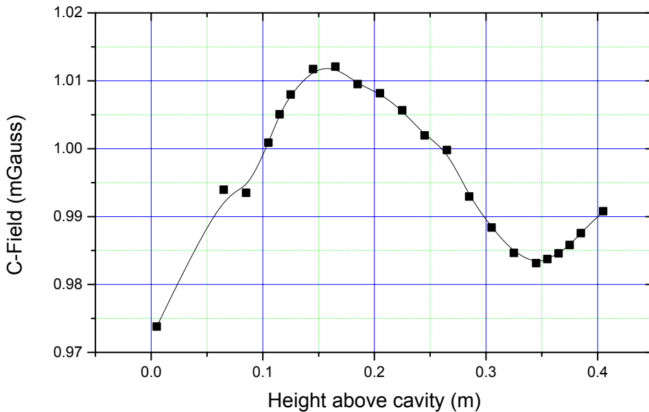
Figure 1. C-field map.
