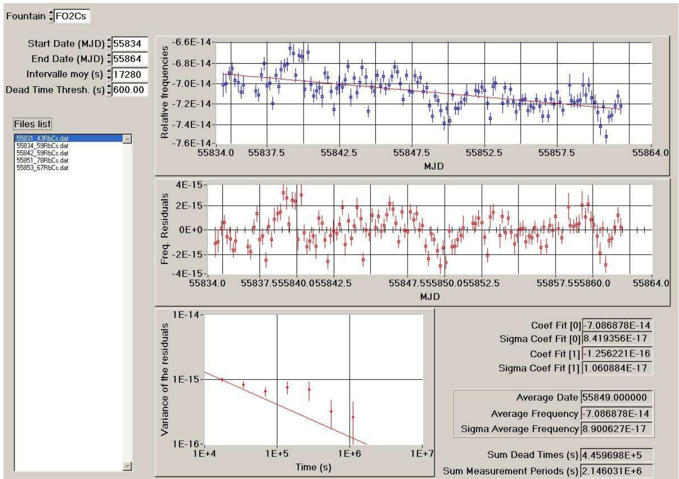
Figure 1: Processing of the data HMaser_{140\ 0890-FO2} for the period MJD 55834-55864
