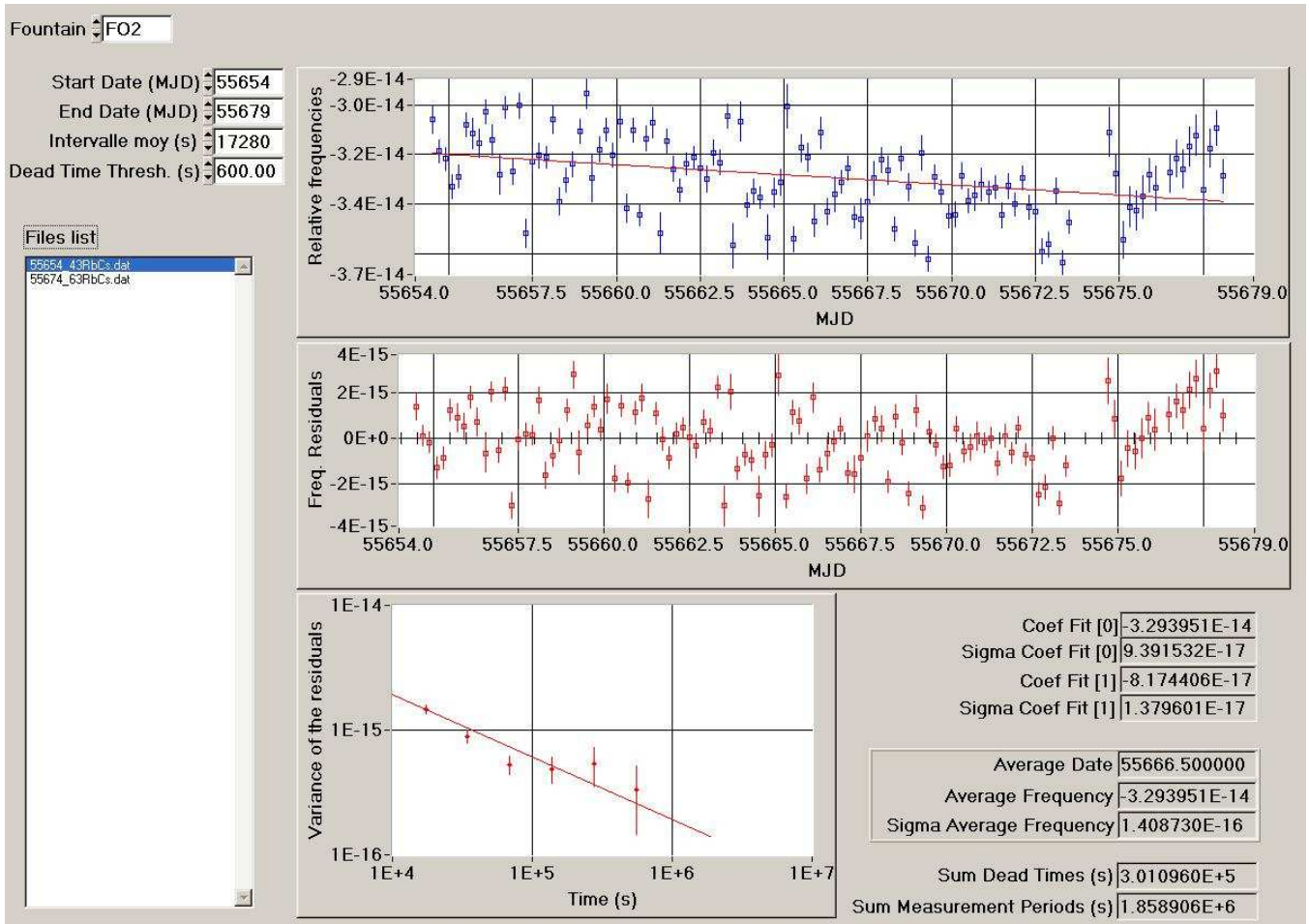
Figure 1: Processing of the data HMaser_{140\ 0890} -FO2 for the period MJD 55654-55679
