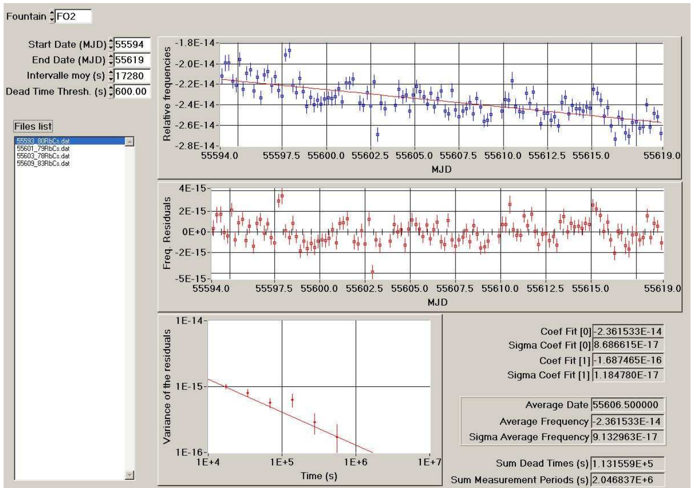
Figure 1: Processing of the data HMaser_{140\ 0890-FO2} for the period MJD 55594-55619
