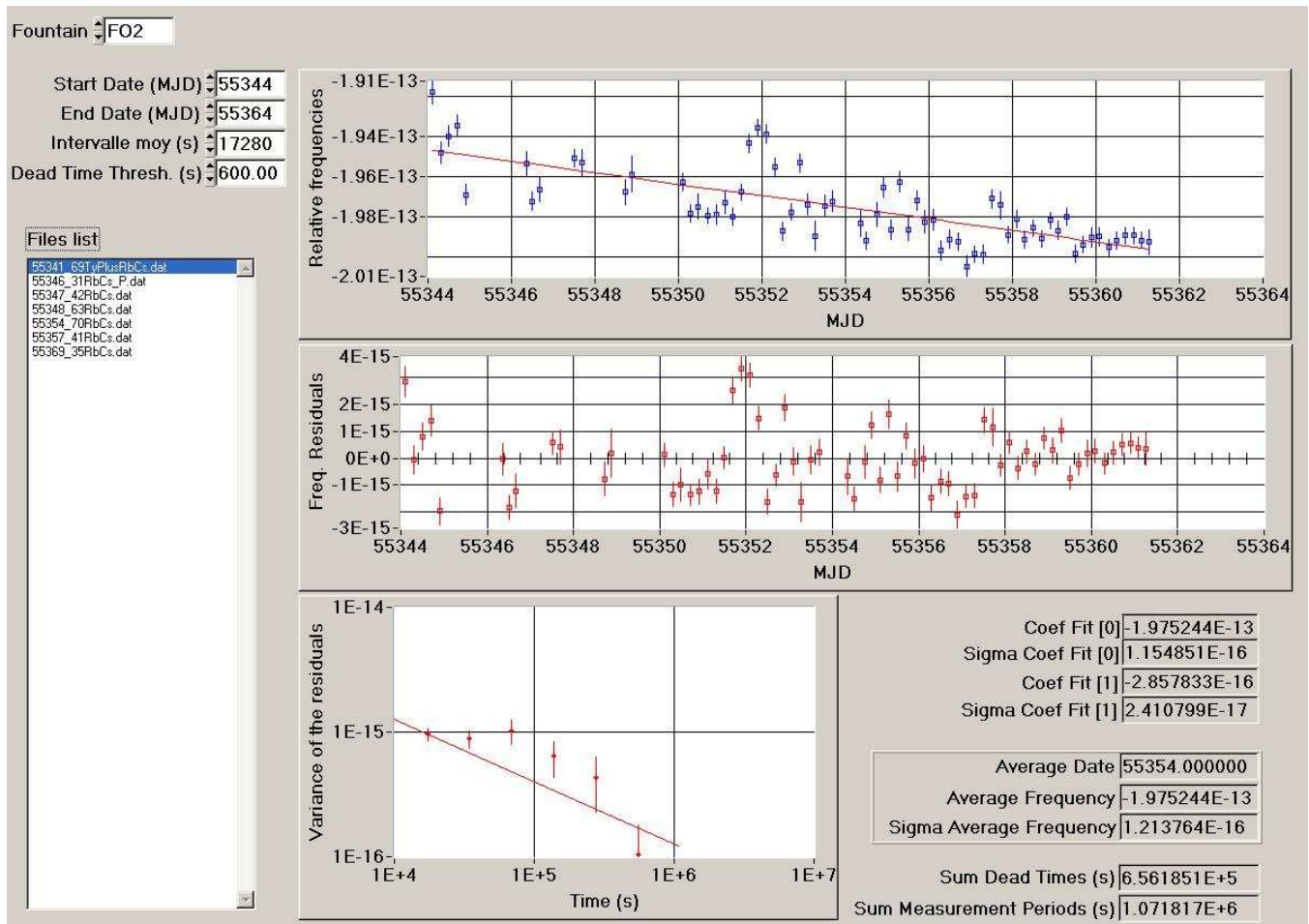
Figure 1: Processing of the data HMaser_{140\ 0890} -FO2 for the period MJD 55344-55364
