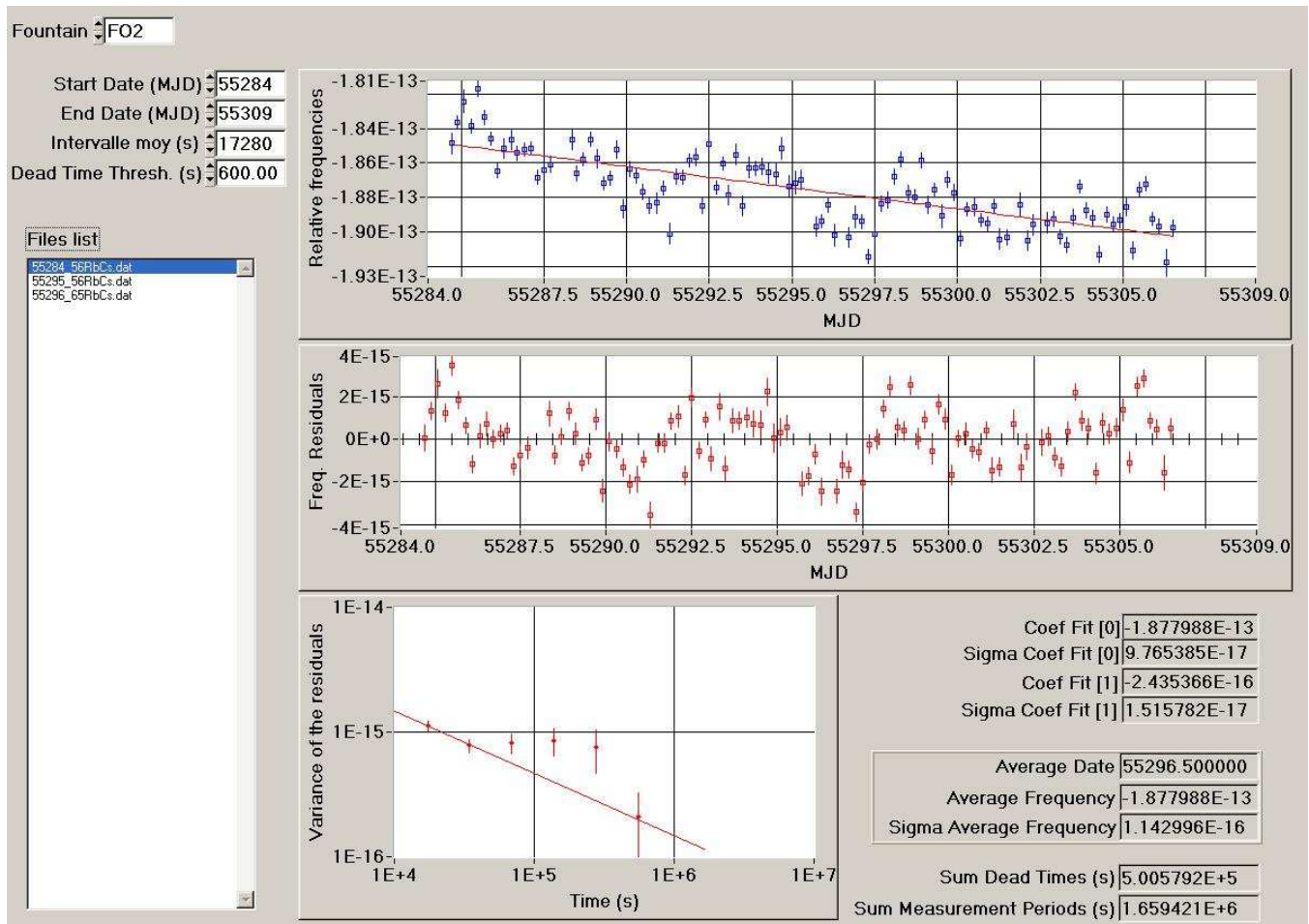
Figure 1: Processing of the data HMaser 140 0890 -FO2 for the period MJD 55284-55309
