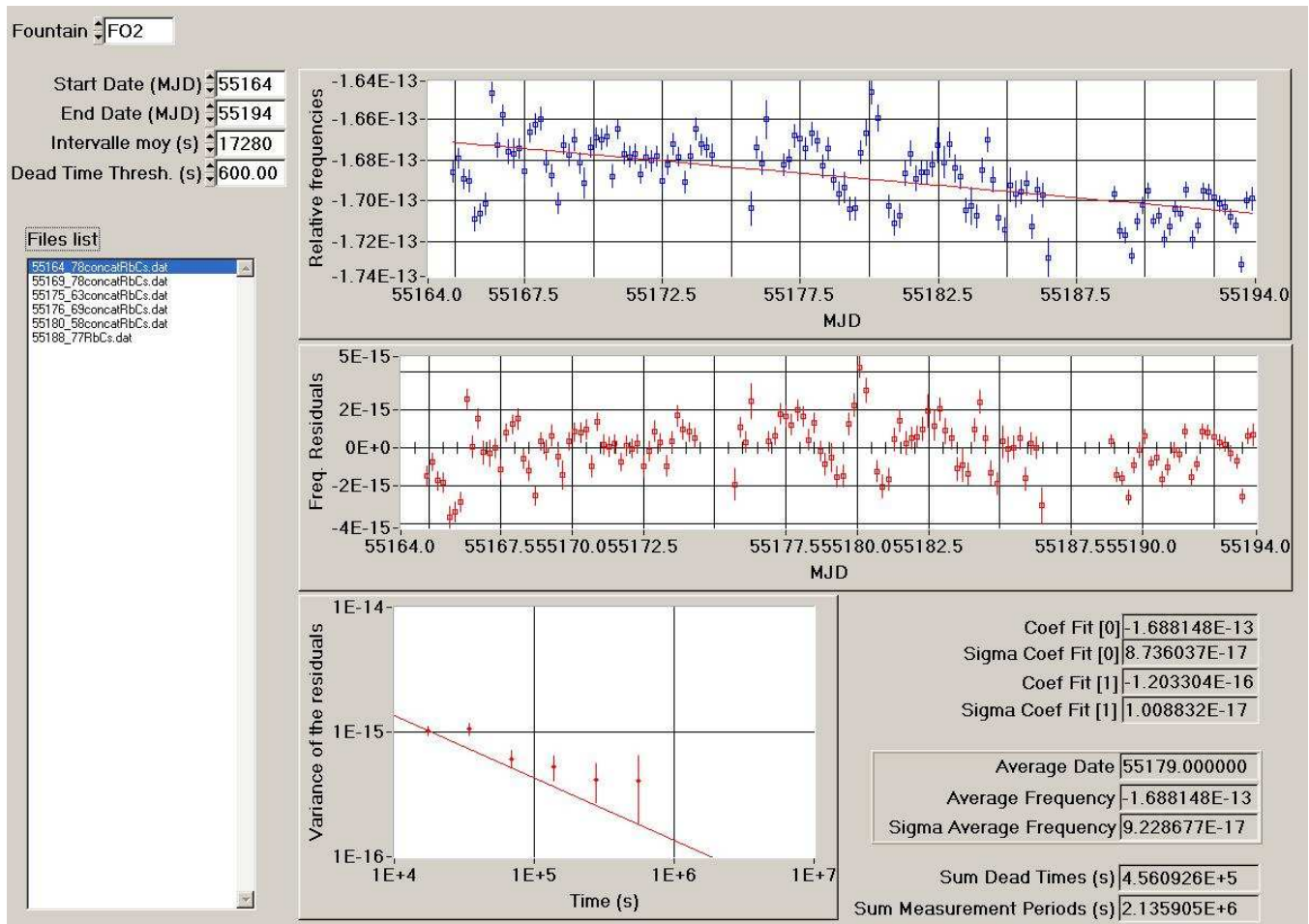
Figure 1: Processing of the data HMaser_{140\ 0890-FO2} for the period MJD 55164-55194
