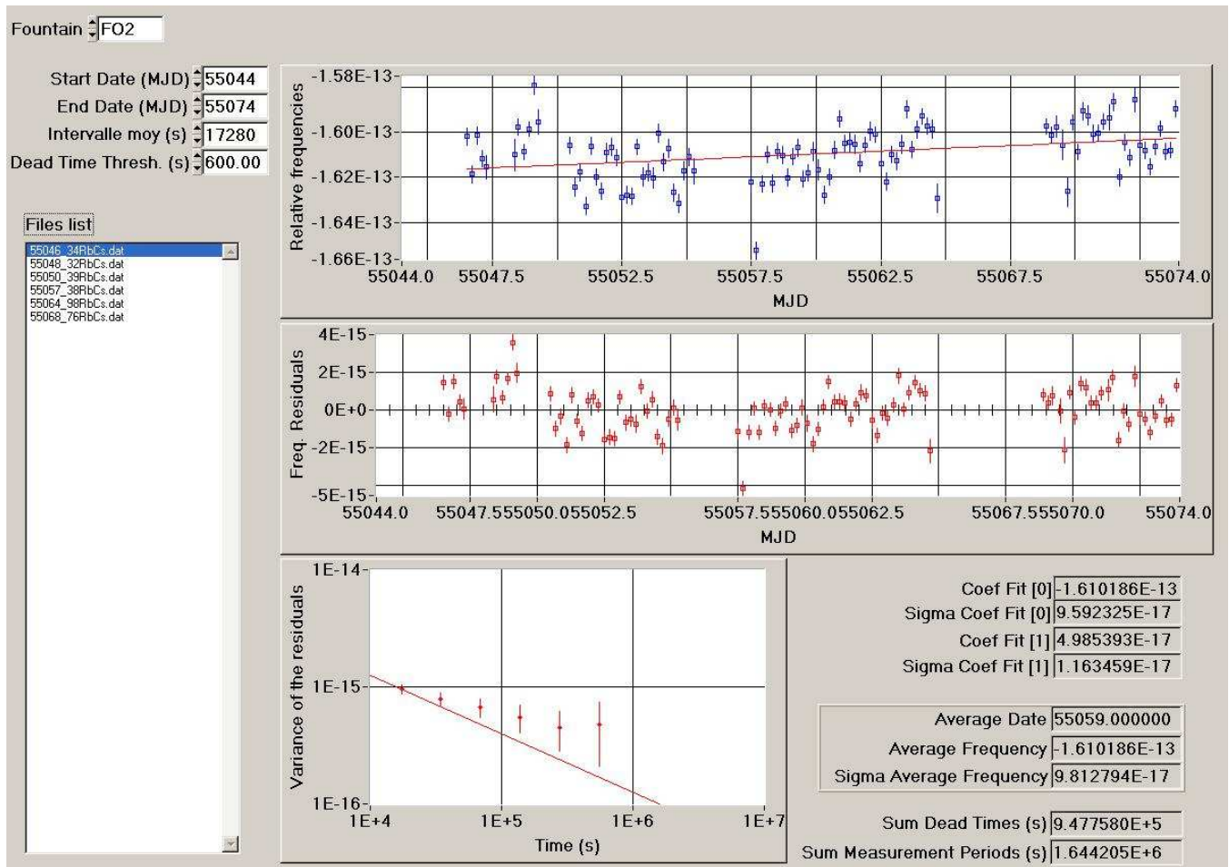
Figure 1: Processing of the data HMaser_{140\ 0890-FO2} for the period MJD 55044-55074
