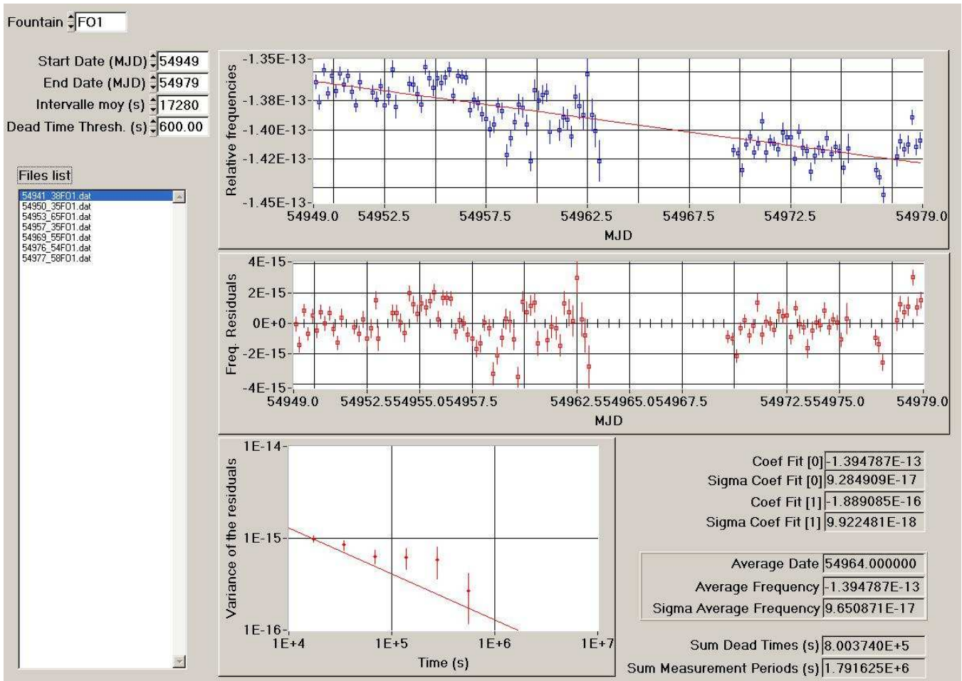
Figure 1: Data processing for the period MJD 54949-54979
