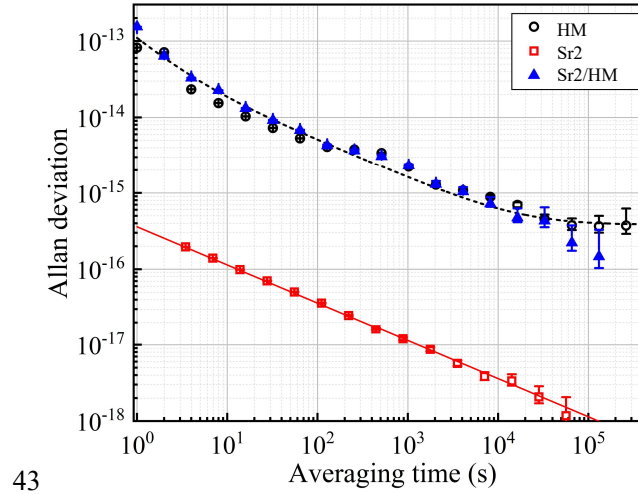
Figure 1. Stabilities of the HM 1415085 and NTSC-Sr2 OLC. The stability of Sr2/HM is determined by the residual values obtained after subtracting the linear fit from the HM frequencies measured by NTSC-Sr2 between MJD 60944 and 60979. The black dashed line shows the HM noise model and the red solid line represents a linear fit of the data with a slope of -0.5.
