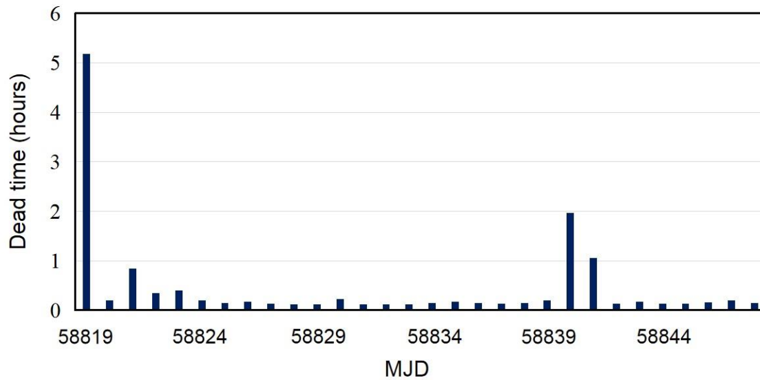
Figure 1 Dead time distributions in Dec., 2019 report period.
