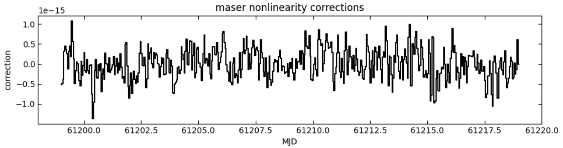
Fig.5. Corrections applied to the assumed frequency of HM 1402014 based on its difference from the ensemble mean. As a correction for instantaneous HM frequency excursions, the overall mean is set to be zero.
