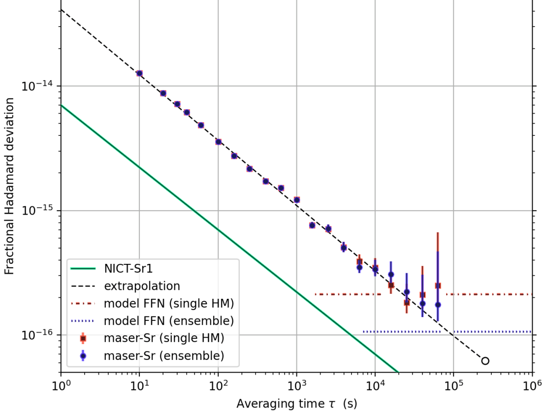
Fig.2. Instability of maser frequency measurements with respect to NICT-Sr1. Blue circles and red squares show the overlapping Hadamard deviation for the residuals from a linear fit with and without correction for deviation of the HM from linear drift, as determined using an ensemble of 4 HMs. Gaps have been removed by contracting the data into a continuous interval. Error bars indicate 1\sigma uncertainties, calculated for white frequency noise. The black dashed line indicates the extrapolation to the full length of available data, used to obtain the statistical uncertainty indicated by the open mark. For long averaging times, the Hadamard deviation falls to a level consistent with the maser stability model, indicated by the red upper dashed line for a single maser, and by the blue lower dashed line for the ensemble, where the instability is expected to improve by a factor of 1/\sqrt{N_{\text{ens}}} . The green line shows the instability contribution from NICT-Sr1.
