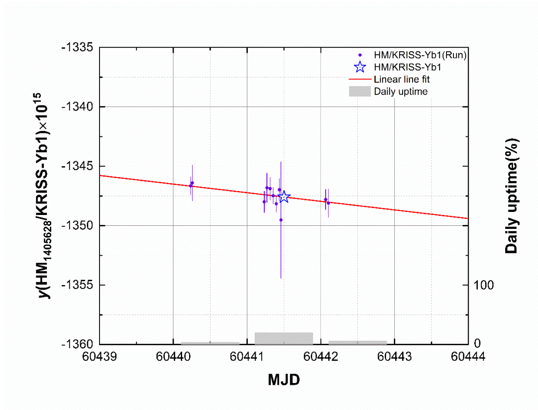
Figure 2. The violet points are averaged data of y(\text{HM}_{1405628}/\text{KRISS-Yb1}) over around 3,600 s with each uncertainty. The blue star indicates the determined value of y(\text{HM}_{1405628}/\text{KRISS-Yb1}) . The red line is the linear fit (drift rate : -0.724 \times 10^{-15}/\text{d} ). The grey bars represent the daily uptime of KRISS-Yb1.
