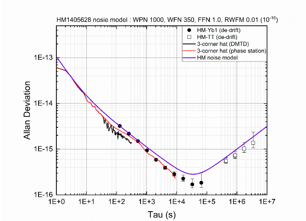
Figure 1. Frequency instability of the hydrogen maser (HM1405628)
