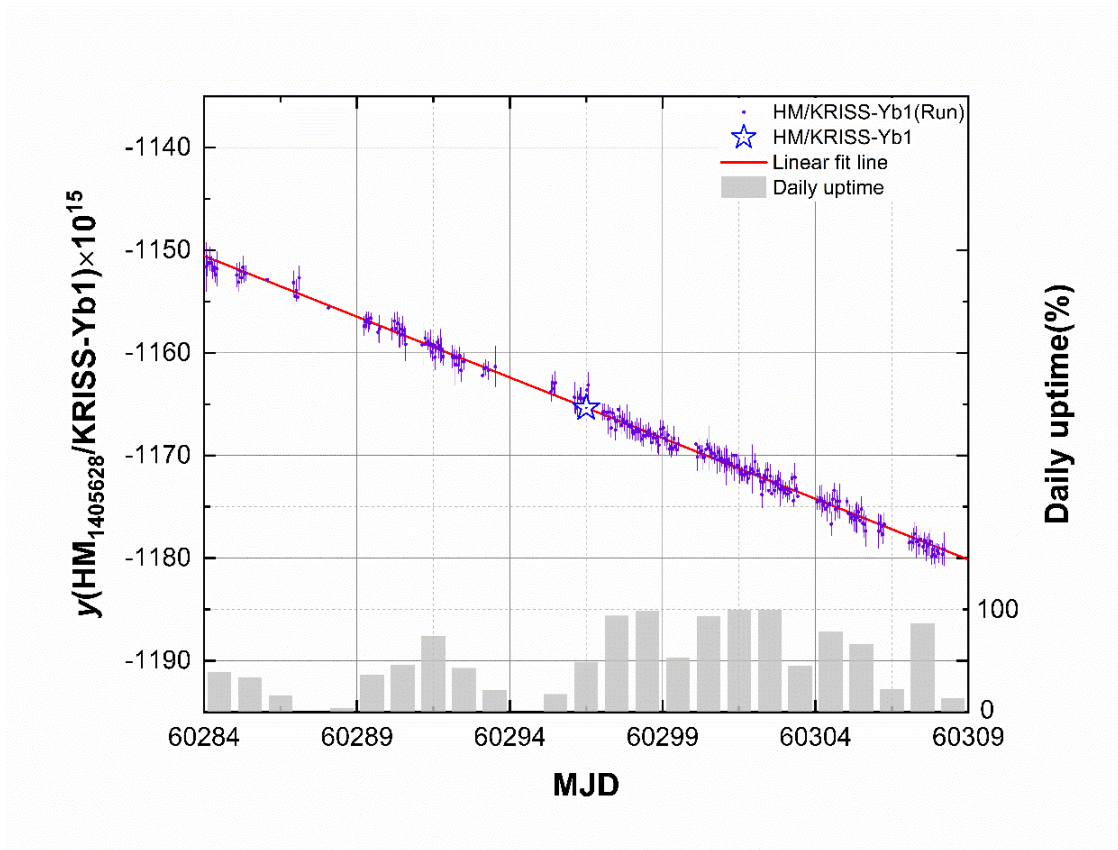
Figure 2. The violet points are averaged data of y(\text{HM}_{1405628}/\text{KRISS-Yb1}) over around 4,000 s with each uncertainty. The blue star indicates the determined value of y(\text{HM}_{1405628}/\text{KRISS-Yb1}) . The red line is the linear fit (drift rate : -1.184 \times 10^{-15}/\text{d} ). The grey bars represent the daily uptime of KRISS-Yb1.
