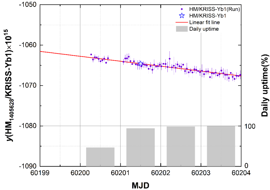
Figure 1. The violet points are averaged data of y(\text{HM}_{1405628}/\text{KRISS-Yb1}) \times 10^{15} over around 4,000 s with each uncertainty. The blue star indicates the determined value of y(\text{HM}_{1405628}/\text{KRISS-Yb1}) . The red line is the linear fit (drift rate : -1.219 \times 10^{-15}/\text{d} ). The grey bars represent the daily uptime of KRISS-Yb1.
