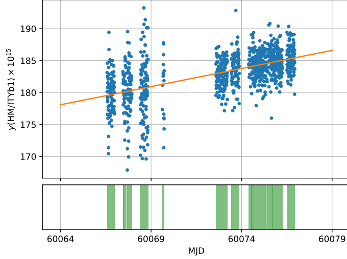
Figure 1: Fractional frequency deviation y(\text{HM1401104}/\text{ITYb1}) measured in the period MJD 60064 - 60079. Green shaded regions in the bottom plot represent the uptime of IT-Yb1.
