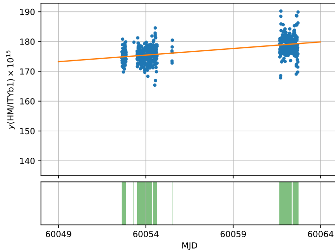
Figure 1: Fractional frequency deviation y(\text{HM1401104}/\text{ITYb1}) measured in the period MJD 60049 - 60064. Green shaded regions in the bottom plot represent the uptime of IT-Yb1.
