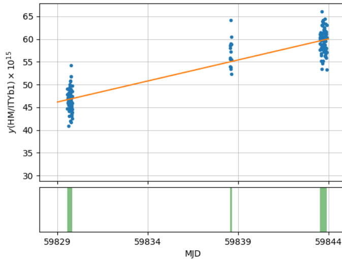
Figure 1: Fractional frequency deviation y(\text{HM1401104}/\text{ITYb1}) measured in the period MJD 59829 - 59844. Green shaded regions in the bottom plot represent the uptime of IT-Yb1.
