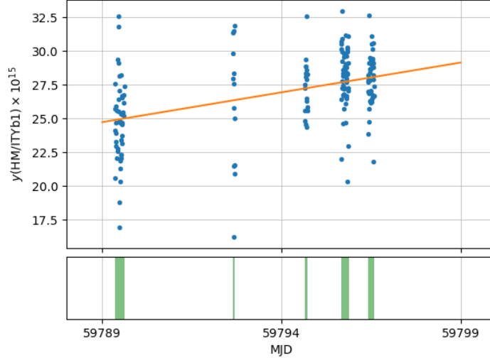
Figure 1: Fractional frequency deviation y(\text{HM1401104}/\text{ITYb1}) measured in the period MJD 59789 - 59799. Green shaded regions in the bottom plot represent the uptime of IT-Yb1.
