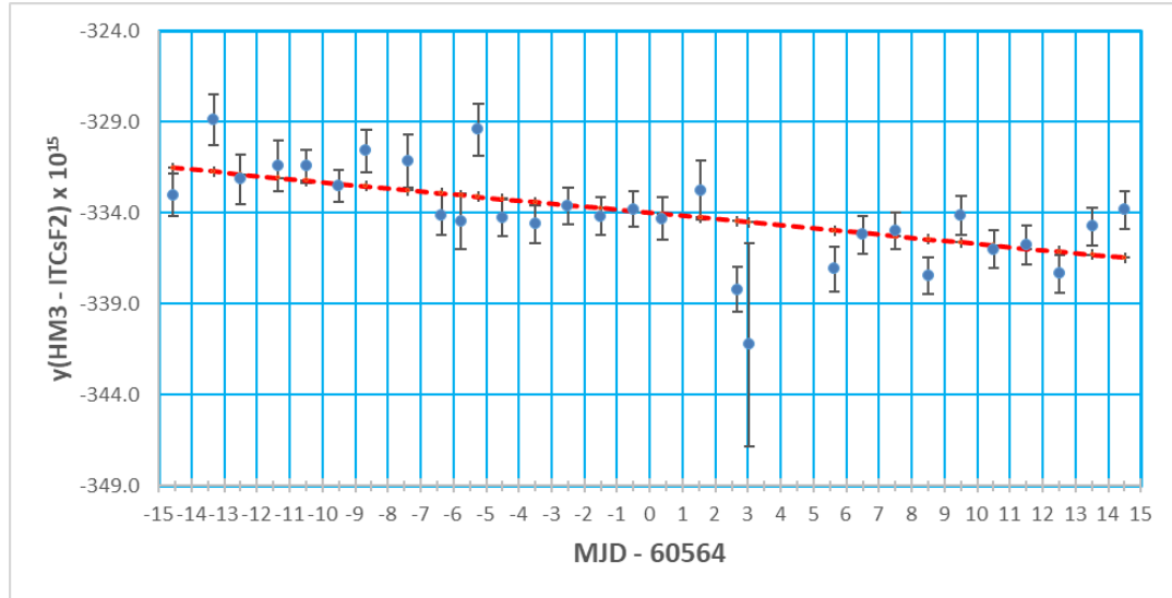
Figure 3. y(HM3-ITCsF2) data and the linear fit curve centered in MJD 60564
