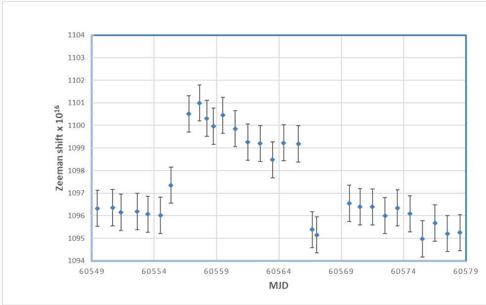
Figure 1. Zeeman shift fluctuations during the TAI evaluation period
