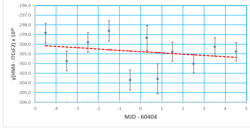
Figure 3. y(HM3-ITCsF2) data and the linear fit curve centered in MJD 60404
