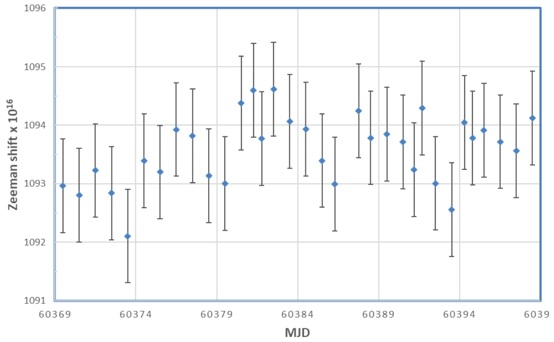
Figure 1. Zeeman shift fluctuations during the TAI evaluation period
