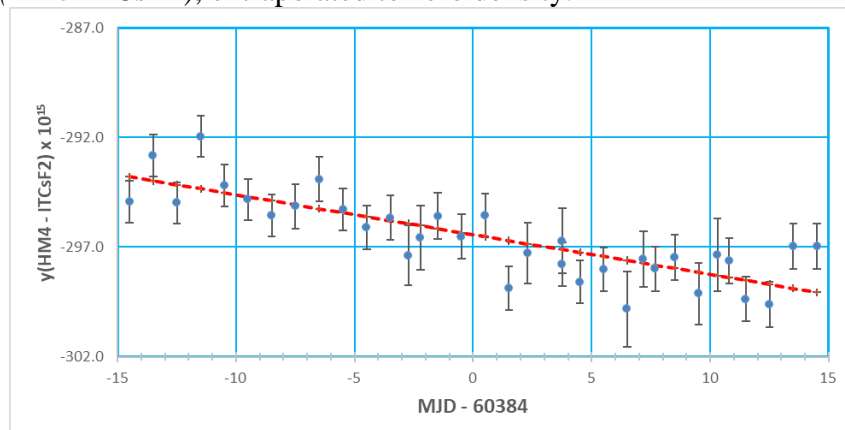
Figure 3. y(\text{HM3-ITCsF2}) data and the linear fit curve centered in MJD 60384
