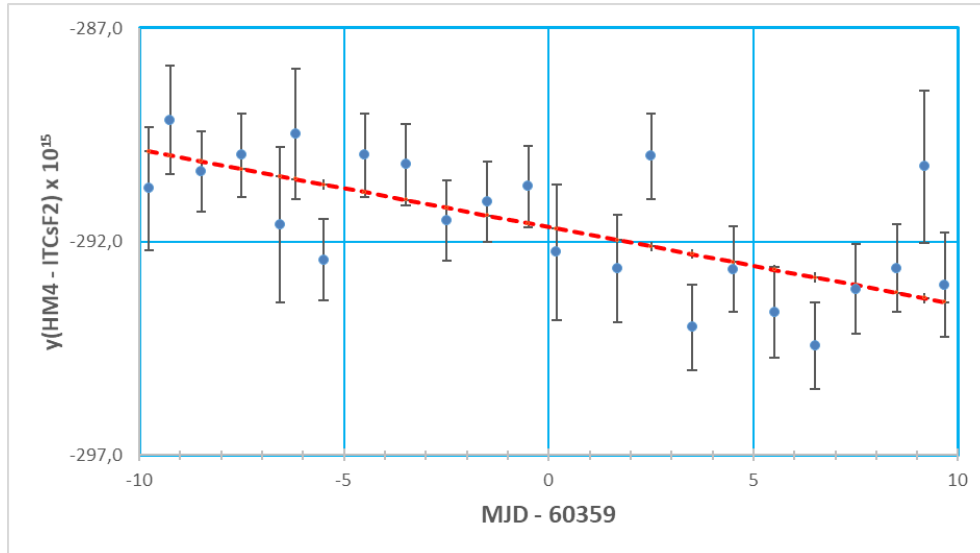
Figure 3. y(HM3-ITCsF2) data and the linear fit curve centered in MJD 60359
